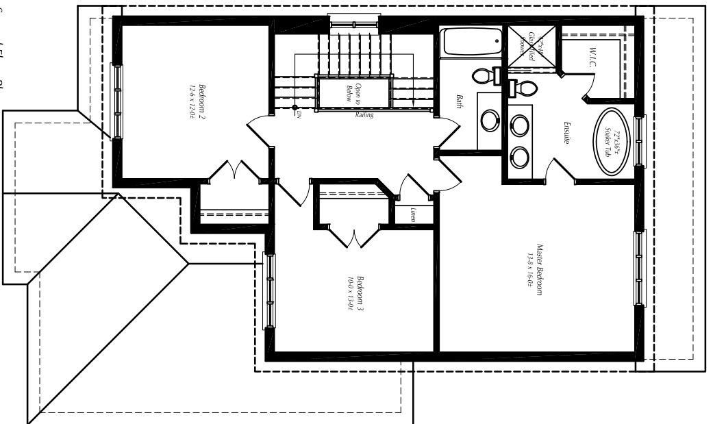
Second Floor Plan (1016 sq.ft.) (Plus 15 sq.ft. Open Space)
