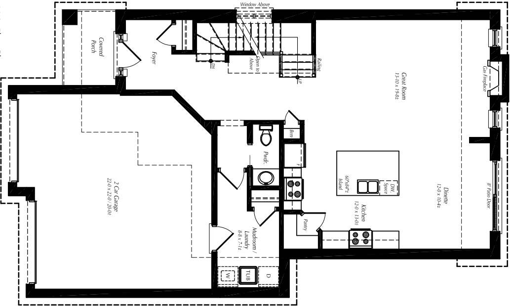
Main Floor Plan (1043 sq.ft.)
