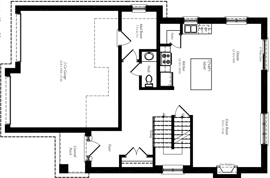
Main Floor Plan (924 sq. ft.)
