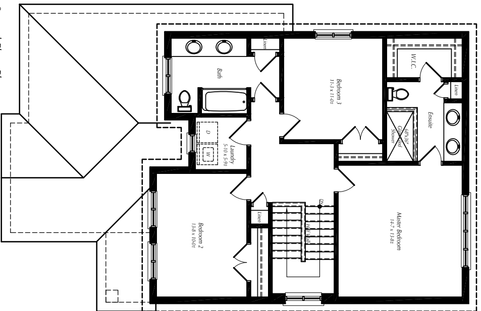
Second Floor Plan (993 sq. ft.)
