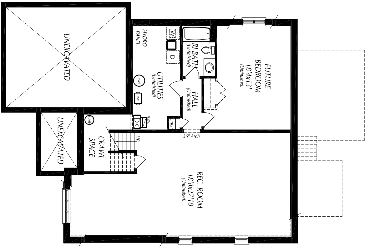
BASEMENT/FOUNDATION PLAN (Unfinished)
