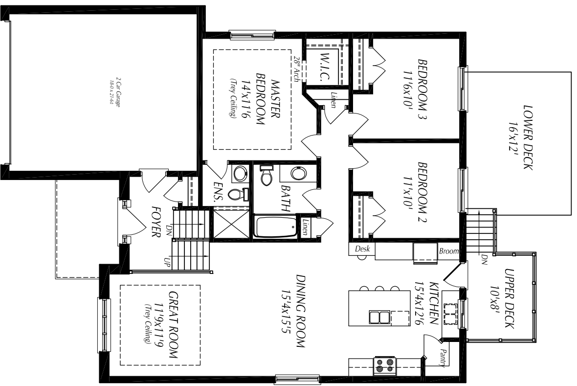
MAIN FLOOR PLAN 1435 sq ft
